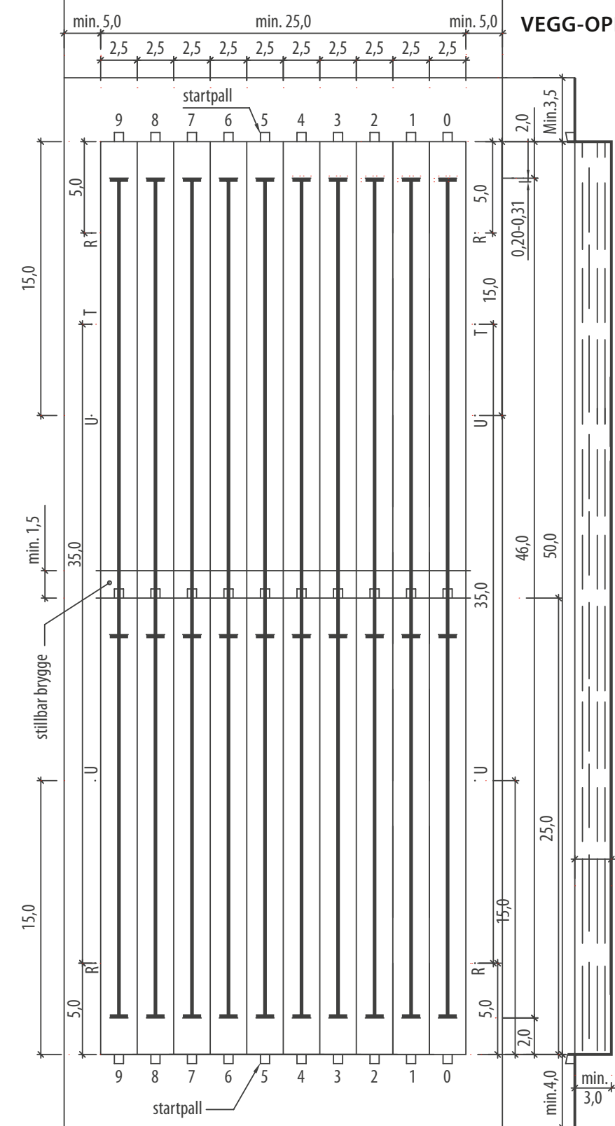
PLAN
