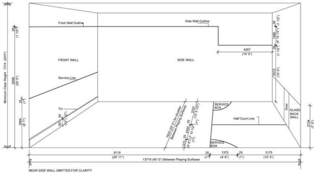
DIAGONALS FOR DOUBLES 15691 (51' 5 3/4") Dimensions of Hardball Doubles Squash Court
